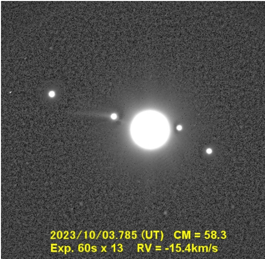
Rank filter
