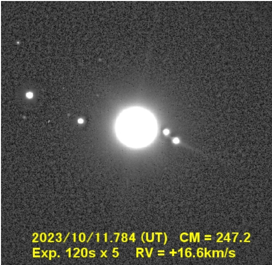
Rank filter
